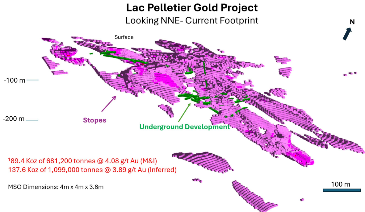
Figure 1: Lac Pelletier representation of underground workings and current resource footprint.
